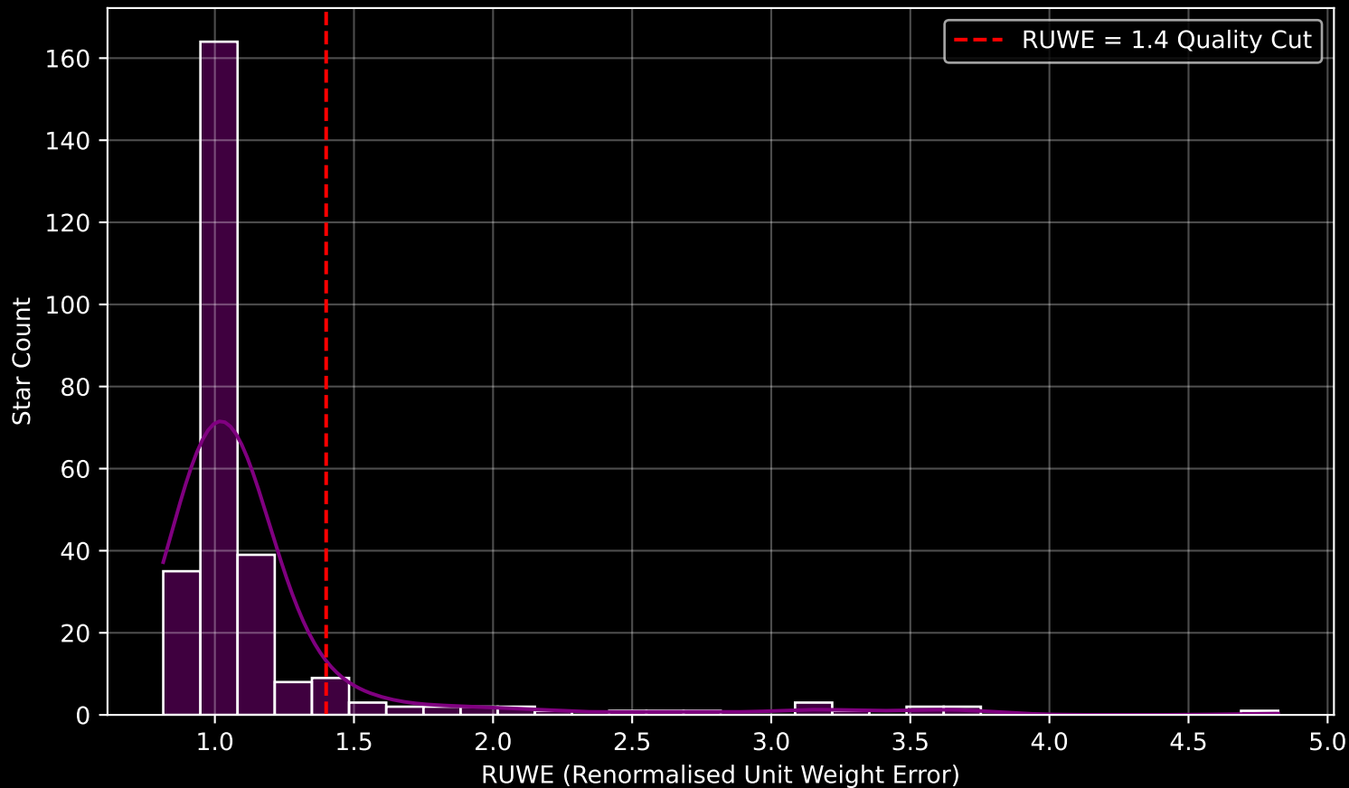
GALAH DR4 Field [411] RUWE Distribution (n= 279)
