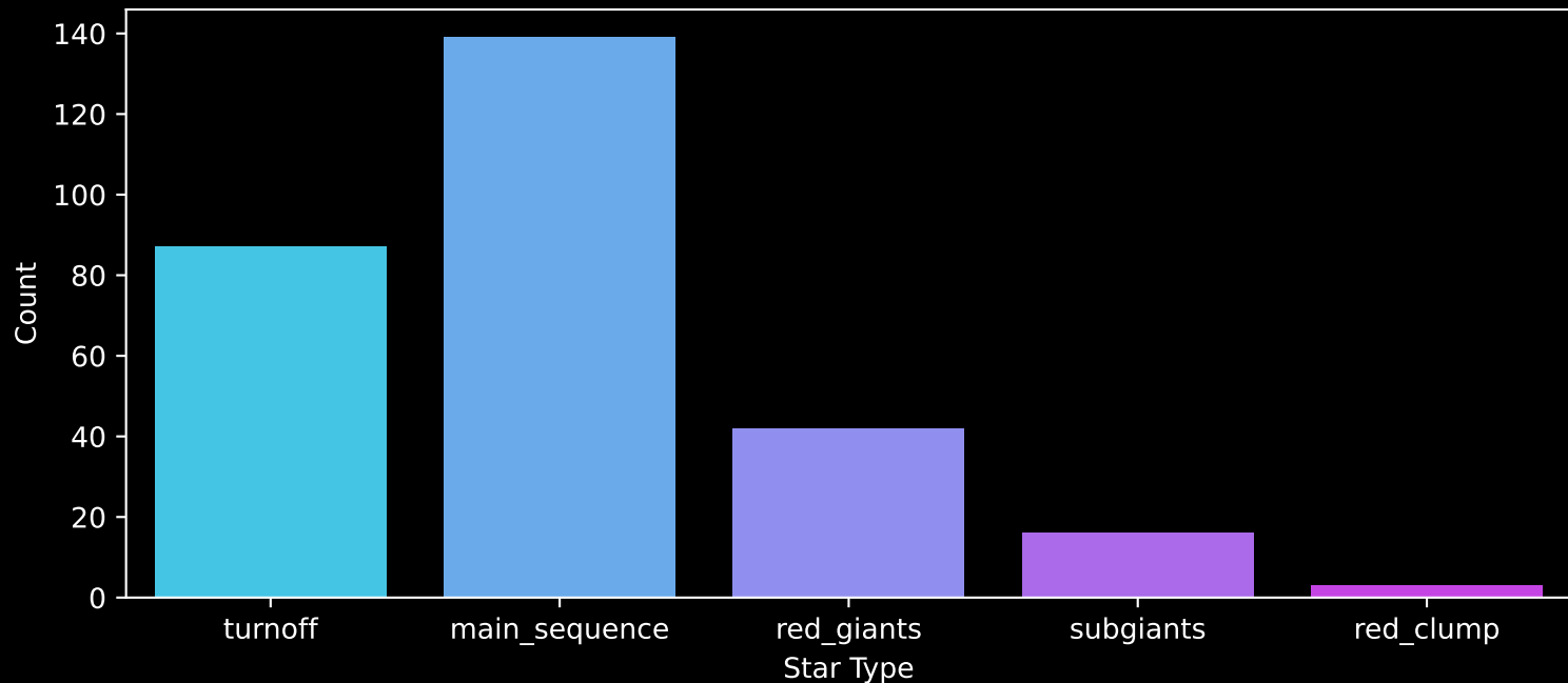
GALAH DR4 Field: [411] Count plot of Star Type
