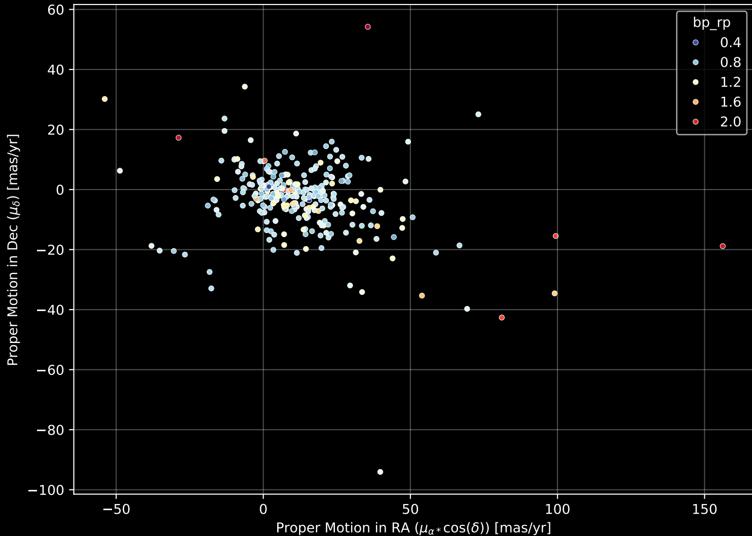
GALAH DR4 Field: [411] Proper Motion Diagram (n= 287)
