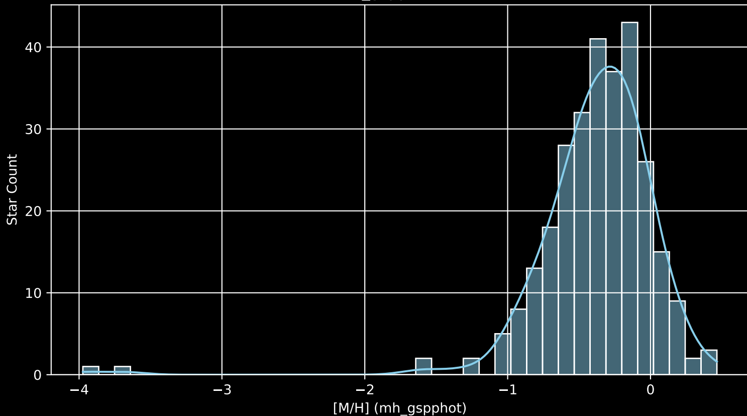
GALAH DR4 Field: [411] [M/H] (mh_gspphot) (n= 286)
