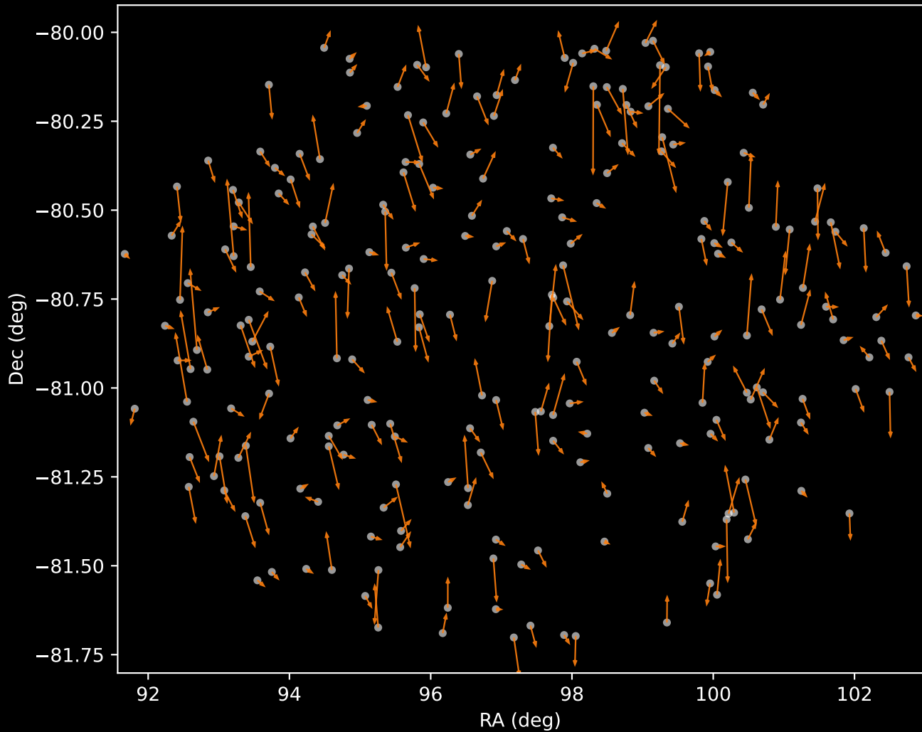
GALAH DR4 Cluster 2 Proper Motion Vectors (n=247)
